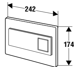
Technical drawing
